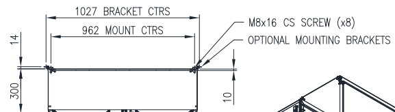
SECTION AW-AW
