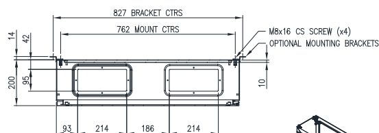
SECTION AW-AW
